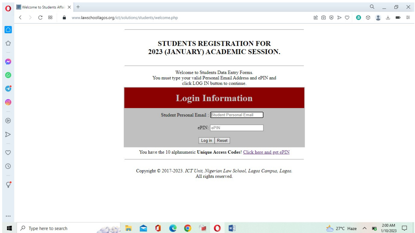
Fig. 2: Welcome/Login page
